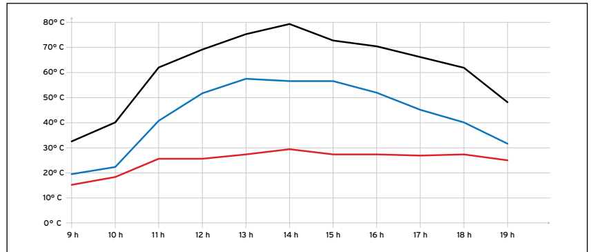
— Outside Temperature — Cool Colours Venezia Black — Standard Material Black
